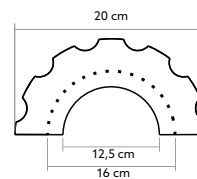
C3002H H: 239,5 cm ProFoam®
